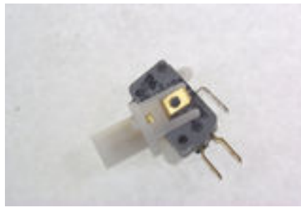
2150.0120 Bulbholder & microswitch for pushbutton
